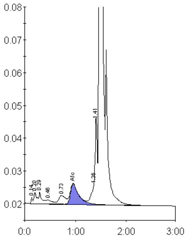
Peak table - ID: 10544892
